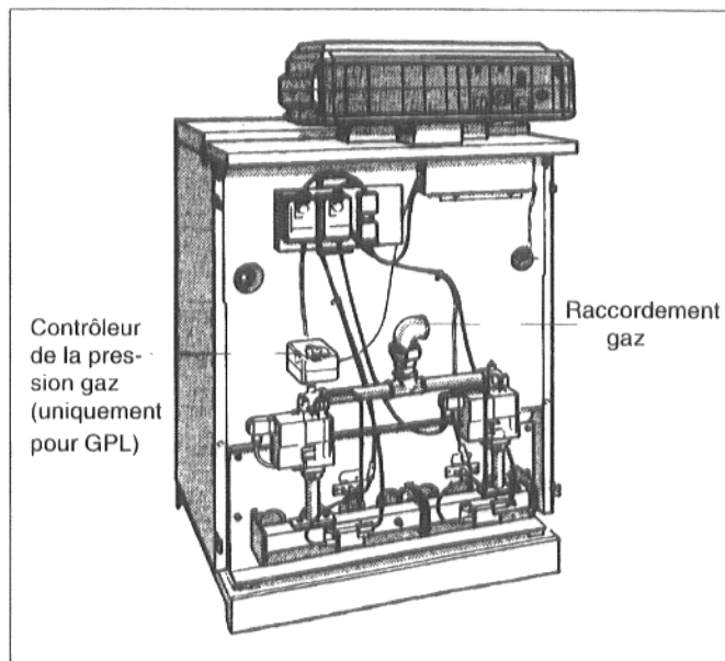
Fig. 23: Raccordement gaz
